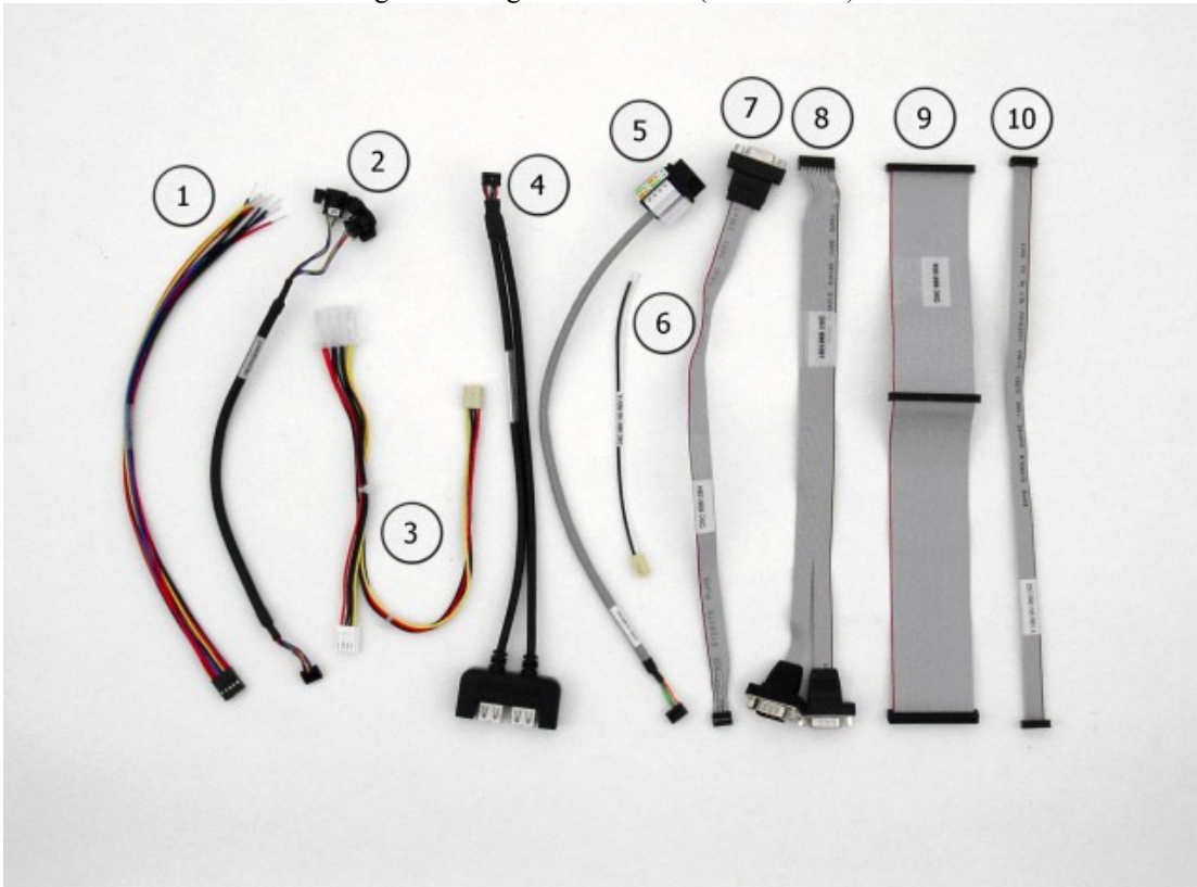
Figure 12: Pegasus Cable Kit (C-PGS-KIT)
